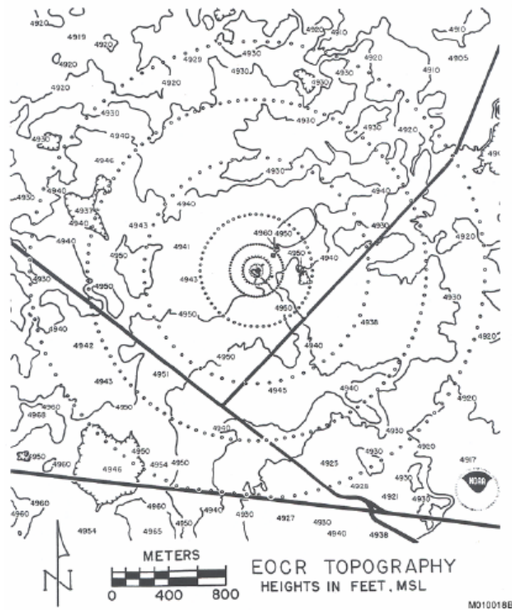
Figure B-6. Terrain map featuring the entire EOCR grid with the source at the grid center (SF 6 releases). Arcs are at distances of about 40, 80, 200, 400, 800, 1200, and 1600 m.
