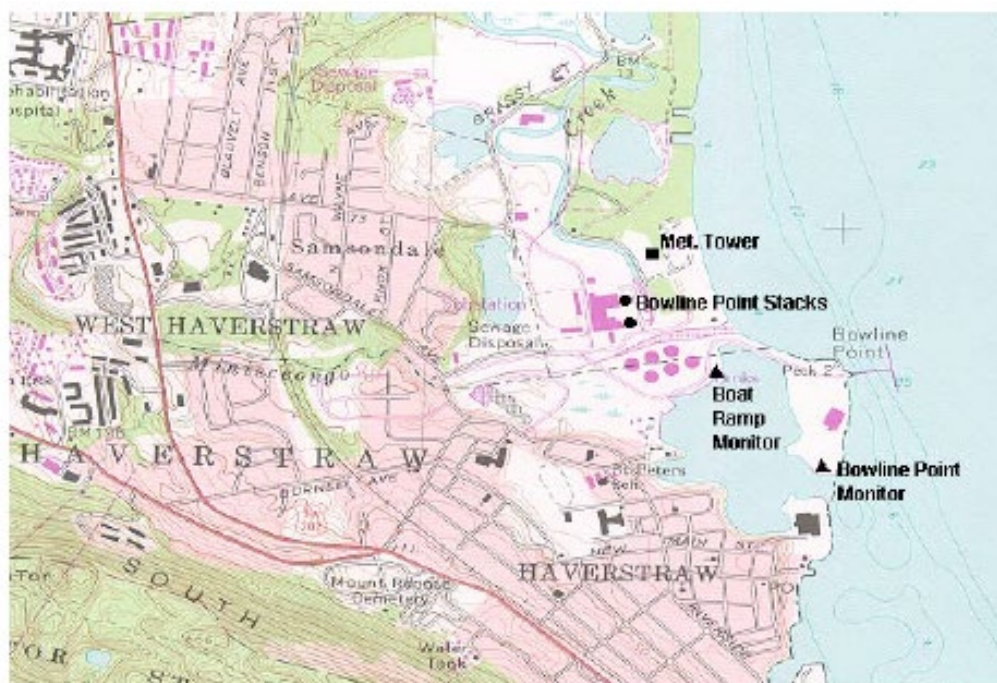
Figure B-13. Bowline Point study area (SO 2 releases)
