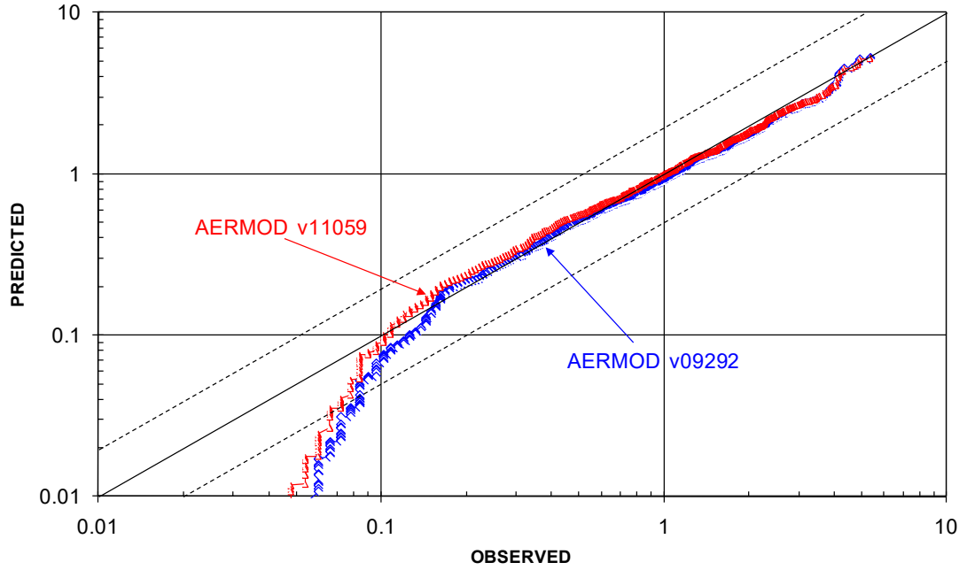
Figure E-1. 1-hour Q-Q Plot for Indianapolis SF 6 Study for All Stabilities
